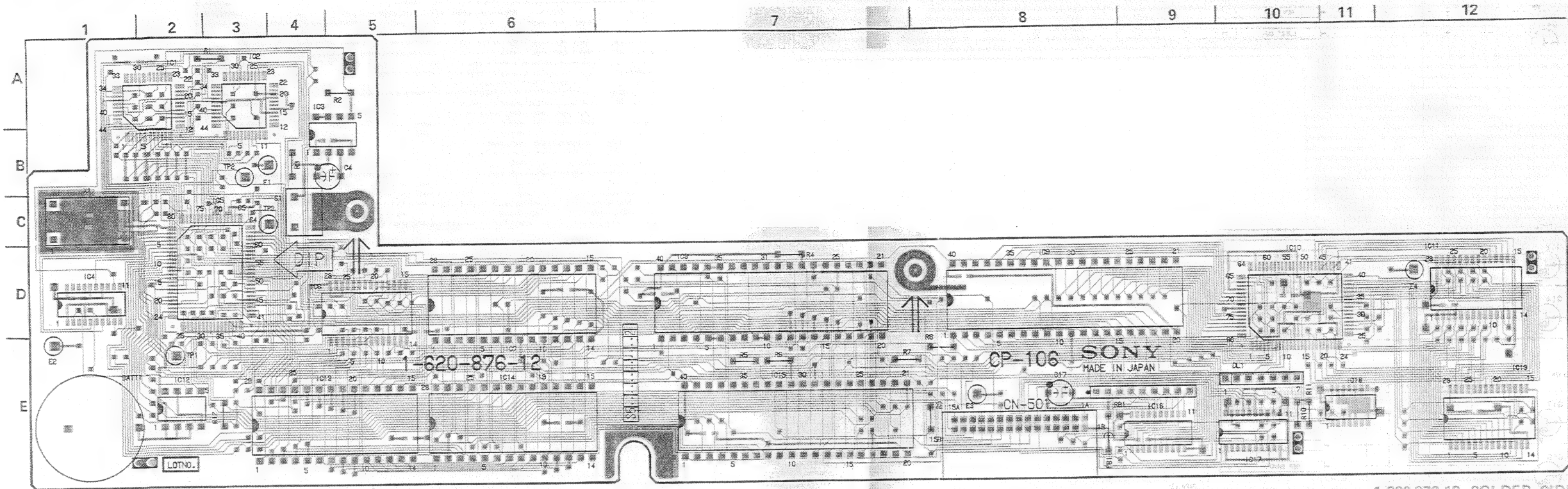
1-620-876-12 COMPONENT SIDE
